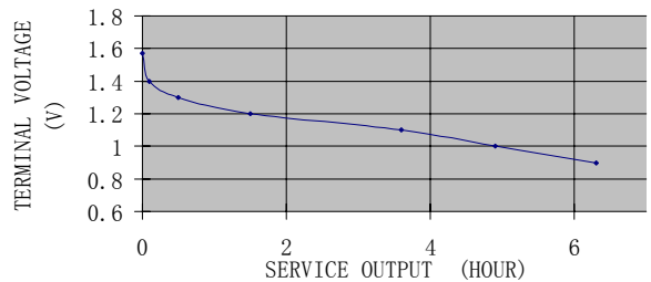
AM-3ALK DISCHARGE CURVE
