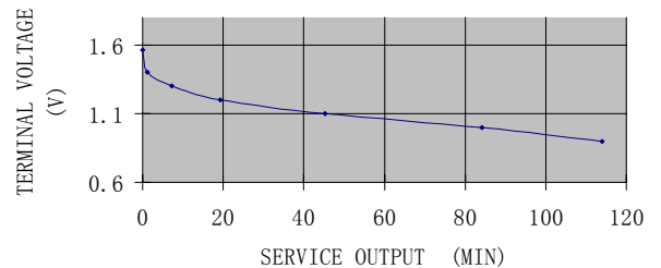
AM-4ALK DISCHARGE CURVE
