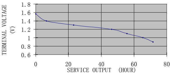
AM-4ALK DISCHARGE CURVE
