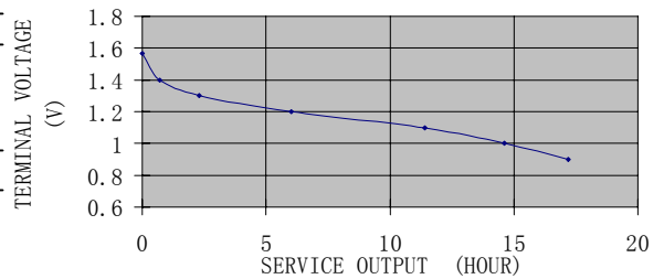
AM-4ALK DISCHARGE CURVE
